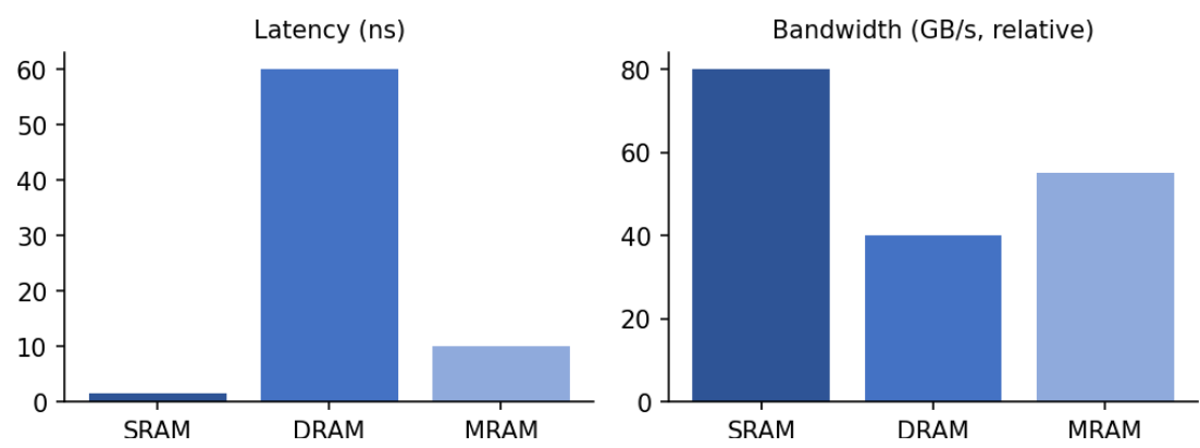
Fig. Q3 — Latency and relative bandwidth: SRAM vs DRAM vs MRAM.
