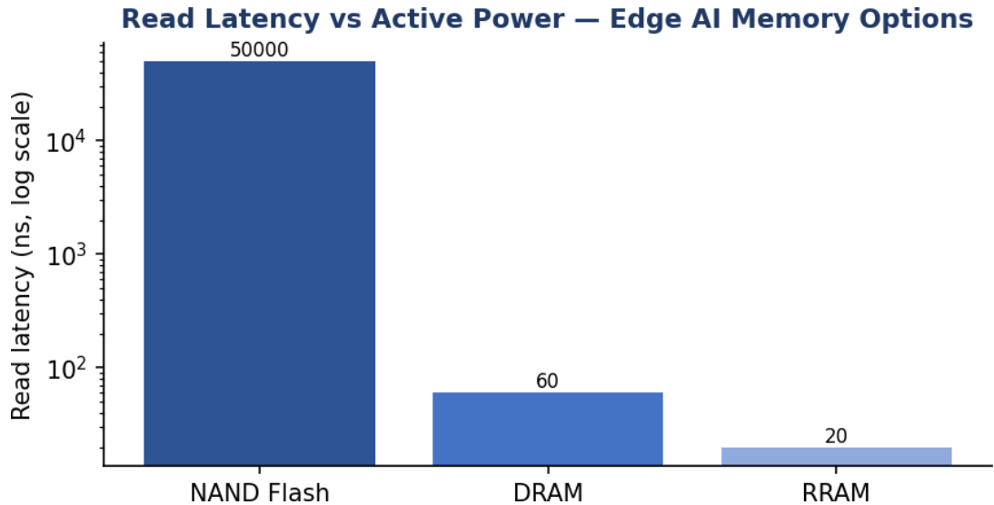
Fig. Q4 — Read latency comparison: NAND Flash vs DRAM vs RRAM (log scale).
